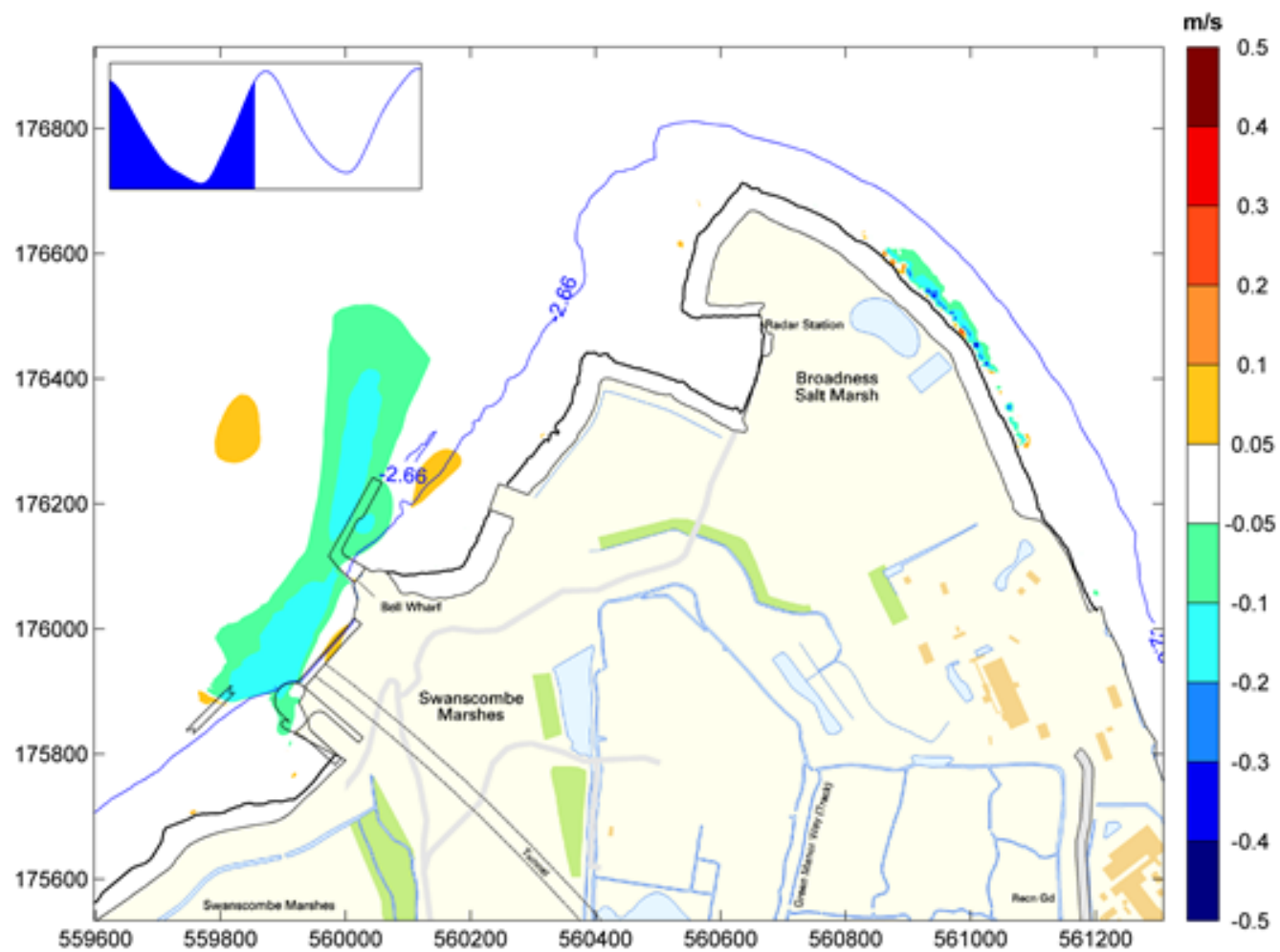
Figure 17.30: Kent Project Site Option C difference in current magnitude at time of peak flood tide against the baseline model.
